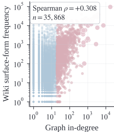
(a) in-degree vs wiki frequency
