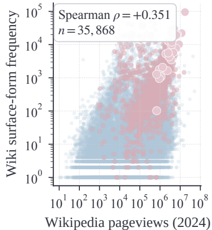
(c) pageviews vs wiki frequency
