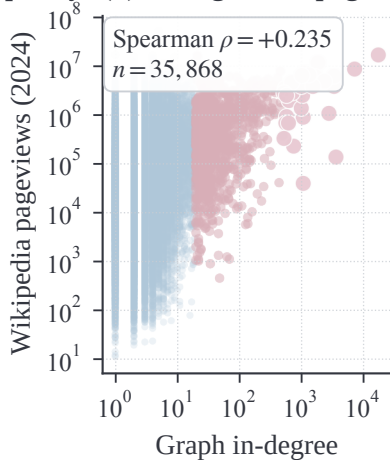
(b) in-degree vs pageviews
